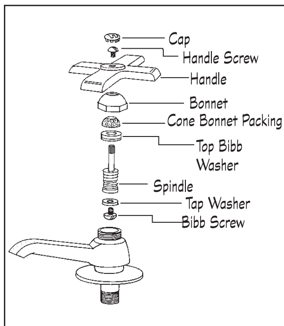
Disassembled faucet.
